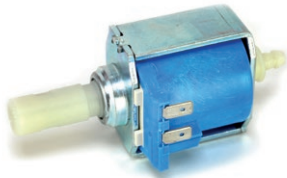
ARS coffee pump Bomba ARS café 65W-20bar
