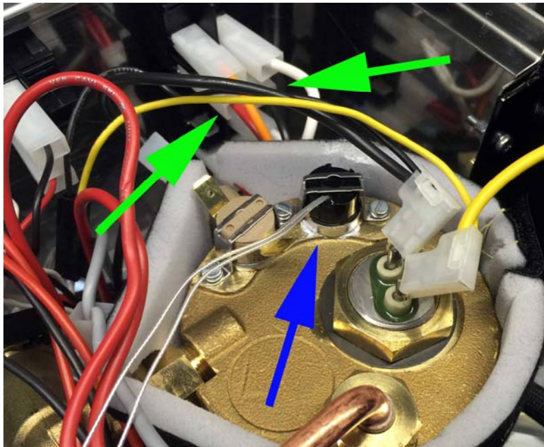
Figure 1. Cables need to be tapped are pointed by green arrows.
